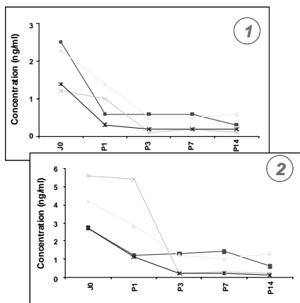
Figure 1: Excretion kinetics for triamcinolone acetone [free fraction (1), total fraction (2)]
