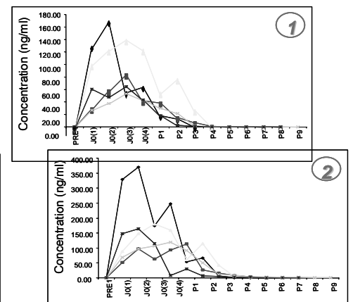
Figure 1: Excretion kinetics for triamcinolone acetone [free fraction (1), total fraction (2)]
