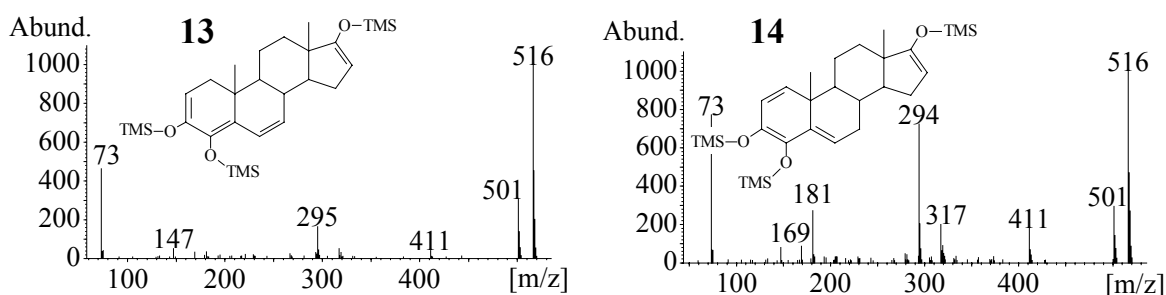
Fig. 11: Mass spectra (EI) of 6,7- ( 13 ) and 1,2-dehydroformestane ( 14 ), per-TMS ( M^+ = 516 )
