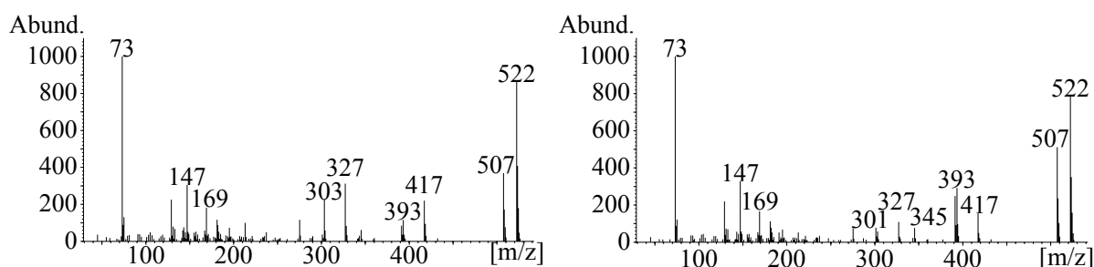
Fig. 4: Mass spectra (EI) of 3,4-dihydroxyandrostan-17-one, per-TMS ( M^+ = 522 ), left: 3 \beta ,4 \alpha ,5 \beta ( 7 ), right: 3 \alpha ,4 \beta ,5 \alpha ( 8 )
